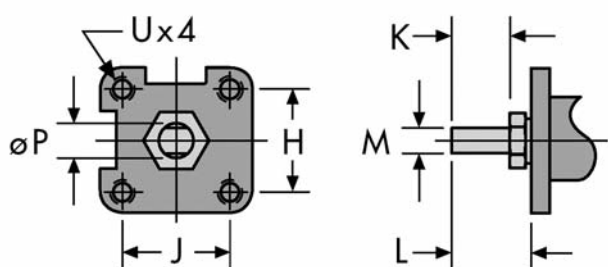
1/4" – 2 1/2" VALVES
