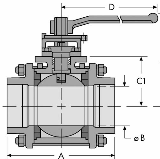
3"–12" VALVES
