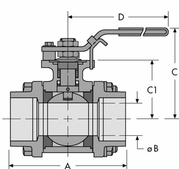
1/2" – 2 1/2" VALVES
